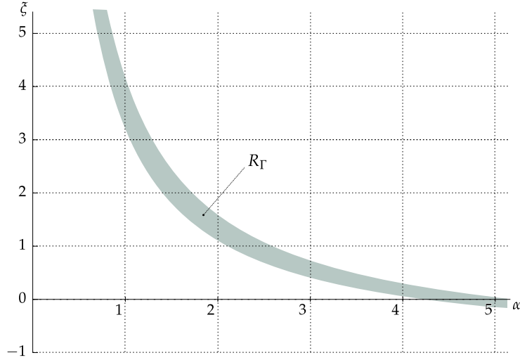
Figure 4: An illustration of set R_\Gamma in the \alpha - \xi plane. Numerical specification is the same as in Figures 2 and 3.
